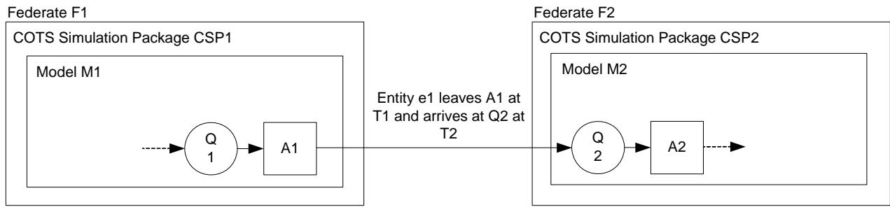
Figure 6-1: IRM Type A.1: General Entity Transfer
