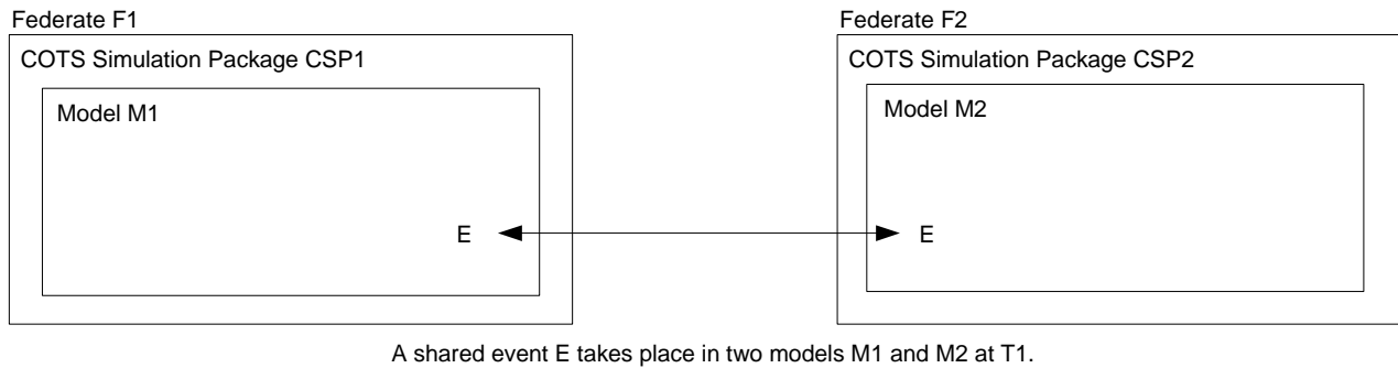
Figure 8-1: IRM Type C.1: General Shared Event
