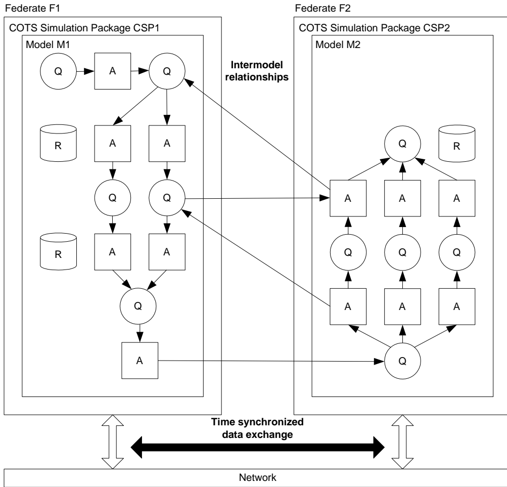
Figure 1-1: The COTS Simulation Package Interoperability Problem
