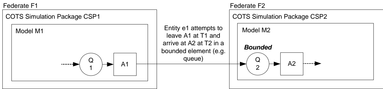
Figure 6-2: IRM Type A.2: Bounded Receiving Element
